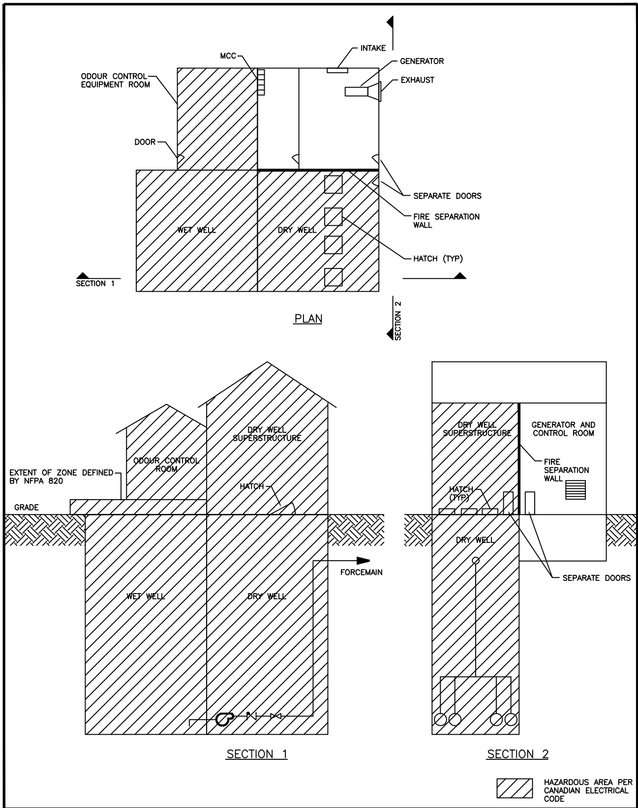
FIGURE 6-6 DESIGN 4 PUMPING STATION HAZARDOUS AREAS
