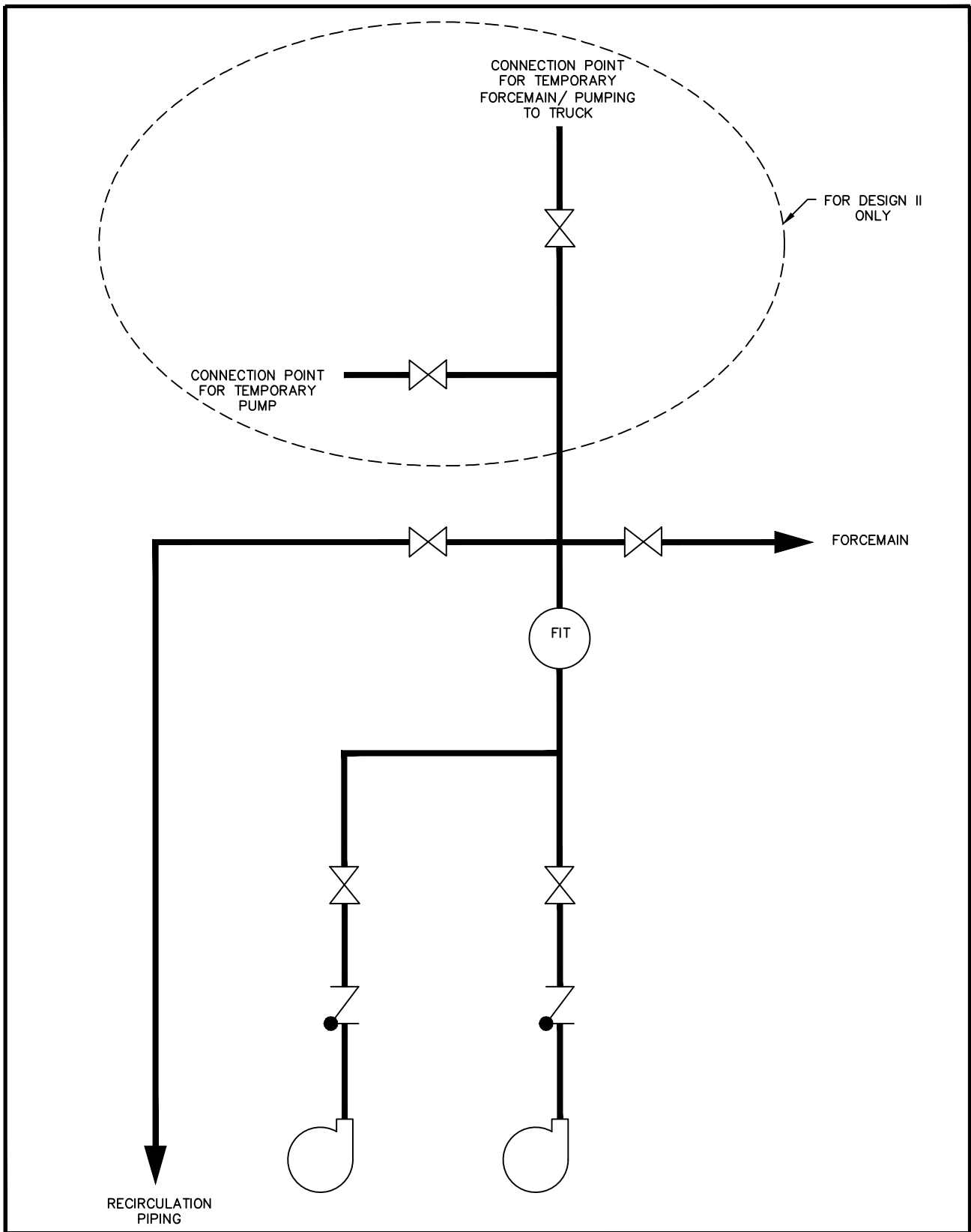
FIGURE 16-1 STATION RECIRCULATION PIPING (DESIGN II, III AND IV)
